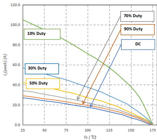
Fig.7-Current Derating
