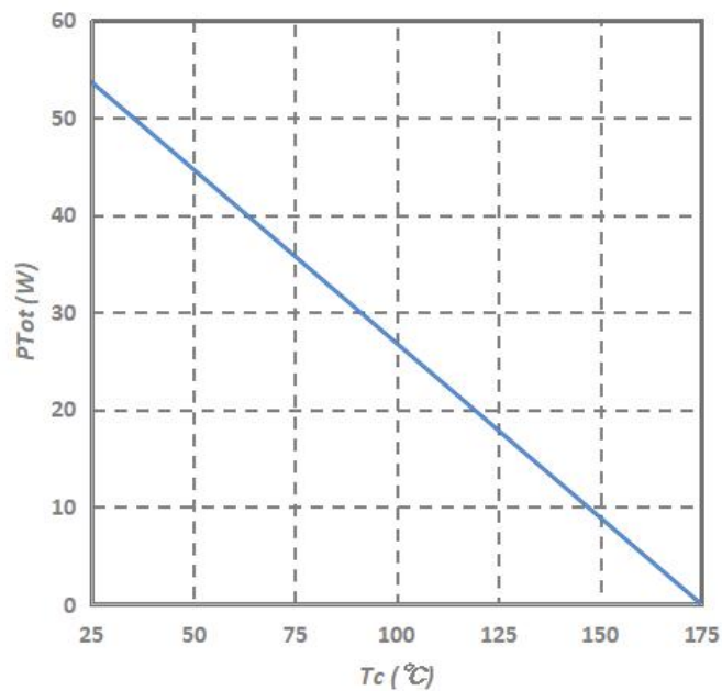
Fig.6-Power Derating
